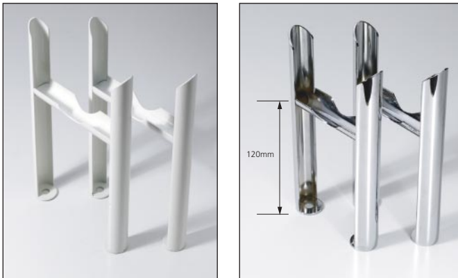
Optional insertable feet - adds 120mm to radiator height
