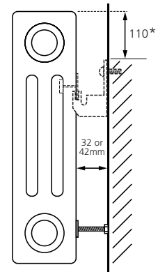
*Recommended bracket fixing position
